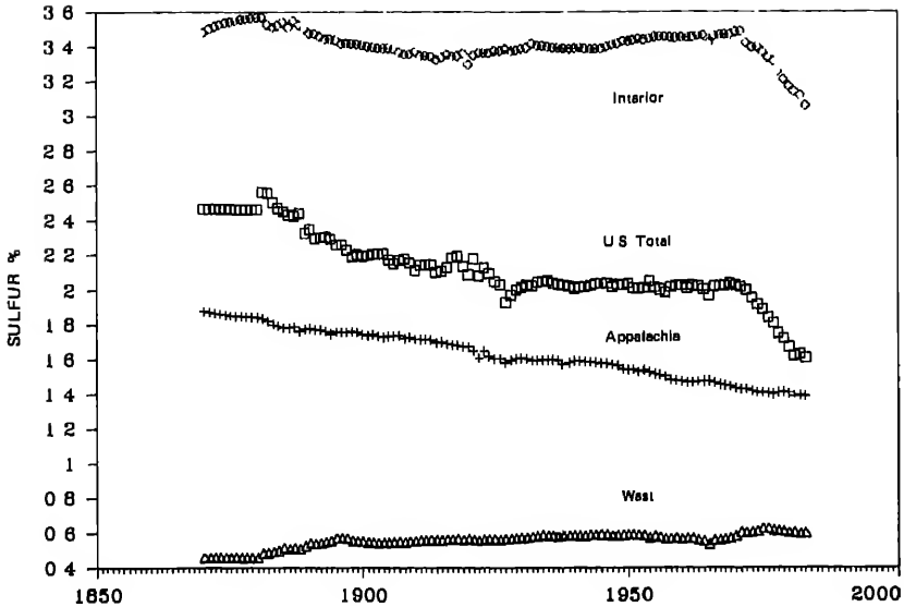
FIGURE 2.12 Trends in the average sulfur content for the Appalachian, Interior, and Western coal-producing regions and the production-weighted aggregate trend for the entire United States.
