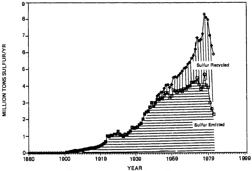
FIGURE 2.21 Trends in sulfur recyclization during petroleum processing and sulfur emissions from petroleum consumption in the United States. Data from Mineral Resources of the United States, Yearbooks (U.S. Geological Survey 1900-1932); Mineral Yearbooks (U.S. Bureau of Mines 1933-1980); Carrales and Martin (1975).
