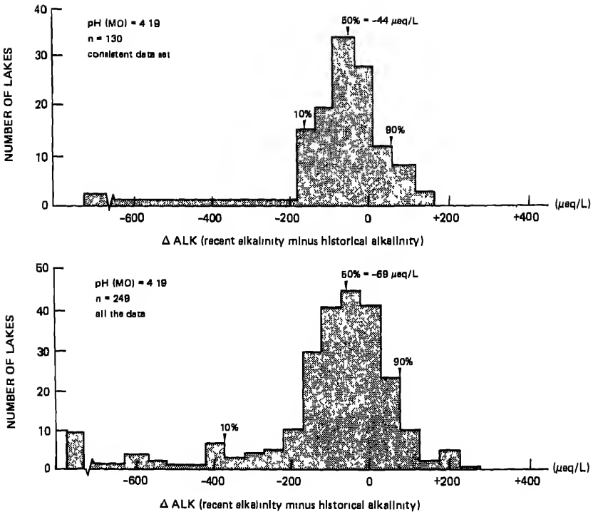
FIGURE 7.15 Plots of change in alkalinities of Adirondack lakes calculated with consistent data only and with all of the data, assuming an endpoint of 4.19. Recent data are from Colquhoun et al. (1984).
