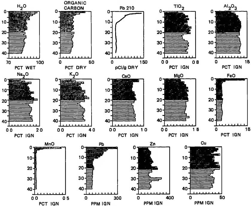
FIGURE 9.24 Sediment chemistry of Lake Husted, Rocky Mountain National Park. The recent increase in lead is indicative of mining activities in the region. See caption, Figure 9.12, for definitions. (From Baron et al. 1984.) Diatom-inferred pH for this sediment core has been stable for at least the past 150 years, fluctuating around 6.6 to 6.8 pH units (see Appendix Table E.5; Beeson 1984).
