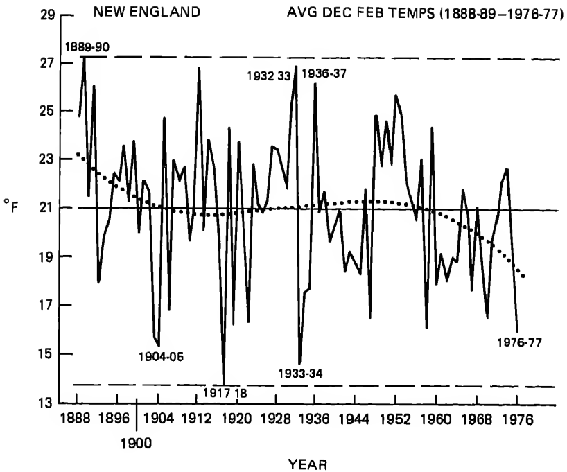
FIGURE 6.12 Trend in winter temperatures in New England (after Diaz and Quayle 1978). The smoothed curve is a third-order polynomial least squares fit.
