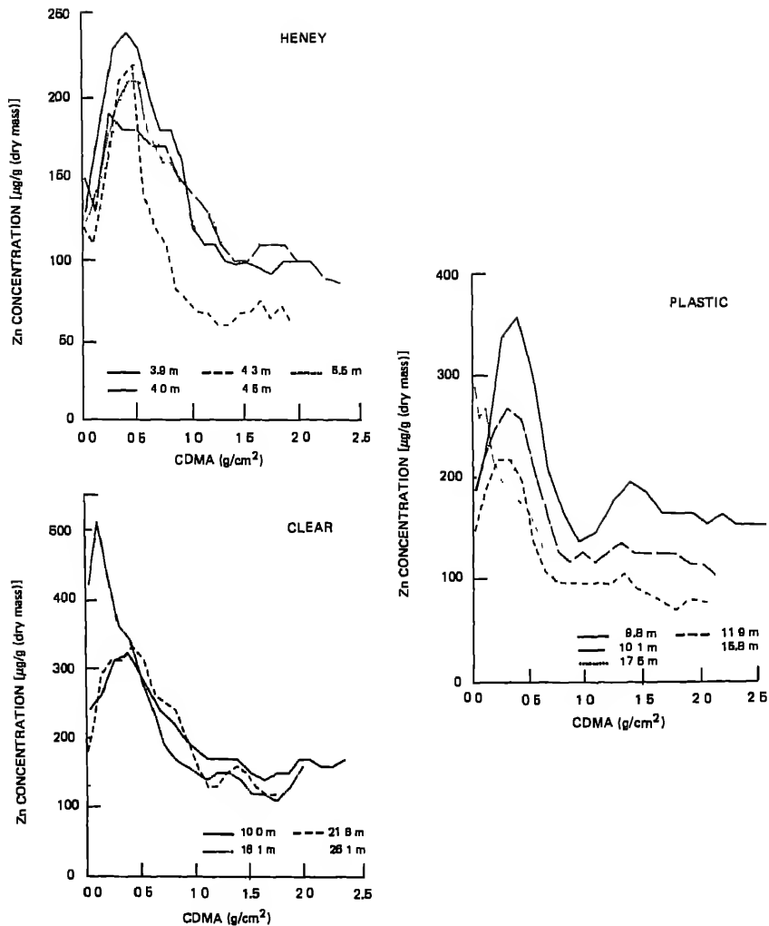
FIGURE 9.14 Zinc concentrations versus CDMA (cumulative dry mass (of sediment) per unit area) (from Evans et al. 1983). CDMA, an alternative way to express depth profile, is employed to take into account sediment compaction. Thus \text{g/cm}^2 corresponds to sediment depth; e.g., the lower the value of CDMA, the more recent the sediment.
