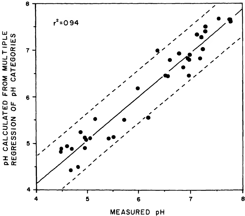
FIGURE 9.2 Predicted lake pH calculated using the equation derived from multiple linear regression of pH categories (assignments based primarily on the distribution of taxa in Adirondack lakes) versus measured surface pH for 37 Adirondack lakes. The dashed lines represent the 95 percent confidence intervals for an individual prediction of pH from diatom data (Charles 1985a).
