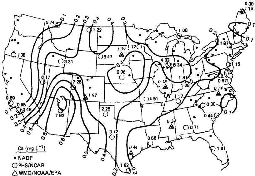
FIGURE 5.16 Weighted average calcium concentration in precipitation (milligrams per liter). The computer-generated contours are for the NADP wet deposition data for 1978-1981 for sites with at least 20 valid samples. The other sites on the map with numerical data show the calcium concentrations determined in earlier years by PHS/NCAR (1960-1966) (bold numbers) and WMO/NOAA/EPA (1972-1973) (italic numbers). SOURCE: Stensland and Semonin (1984).
