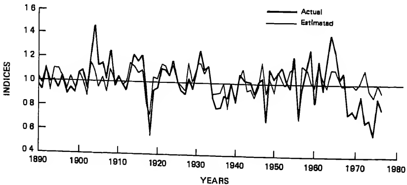
FIGURE 6.11 Actual and estimated red spruce tree ring indices at Lake Arnold in the Adirondack Mountains (elevation 1150 m) based on a temperature response model. The model was developed using mean daily temperatures for the Northern Plateau Climatic Division of New York. The model was calibrated using the 1890-1950 period, and model predictions run from 1951 to 1976. The dark line is the actual indice record, the light line is the estimated indice record. The climate model was \text{Index} = -0.261 Jp - 0.300 Ap + 0.180 Op + 0.202 Np + 0.291 Dp + 0.155 Mc + 0.209 Sc . R^2 = 0.502 ; R_{\text{adj}}^2 = 0.436 , DF = 53 . ( Jp , previous July temperature; A, August; N, November; D, December; Mc, current May temperature; S, September). (From Cook 1985). The number of rings at breast height ranged from 142 to 297, with most in the range 200 to 250.
