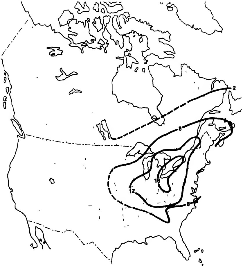
FIGURE 5.13 Enrichment factors for sulfate concentrations in North American precipitation. Numbers signify the ratio of sulfate concentration in precipitation in eastern North America to sulfate concentration in precipitation in remote areas of the world. SOURCE: Galloway et al. (1984).
