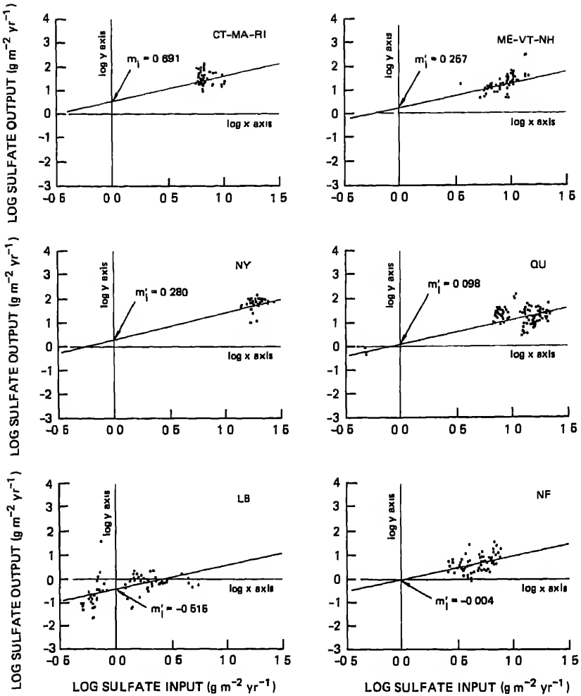
FIGURE 7.3 Regional relationships between inputs and outputs of sulfate for lakes in northeastern North America assuming that the only source of sulfate input is from wet deposition.
