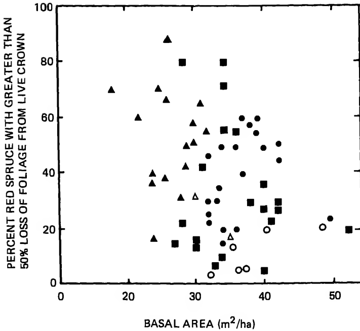
FIGURE 6.6 Percent red spruce in an advanced state of deterioration versus stand basal area. Data correspond to spruce in categories 3 and 4 (Table A.1). Filled circles, Mount Washington, New Hampshire; filled triangles, Mount Mansfield, Vermont; filled squares, Whiteface Mountain, New York; open triangles, Catskill Mountains, New York; open circles, southern Appalachian sites.
