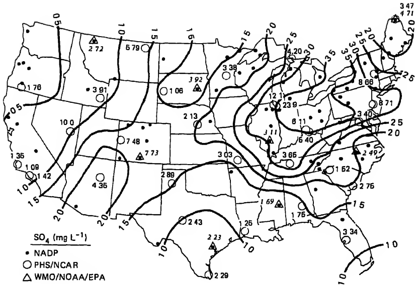
FIGURE 5.17 Weighted-average sulfate concentration in precipitation (milligrams per liter). The computer-generated contours are for the NADP wet deposition data for 1978-1981 for sites with at least 20 valid samples. The other sites on the map with numerical data show the sulfate concentrations determined in earlier years by PHS/NCAR (1960-1966) (bold numbers) and WMO/NOAA/EPA (1972-1973) (italic numbers). SOURCE: Stensland and Semonin (1984).
