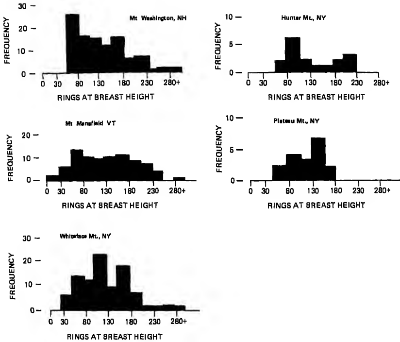
FIGURE 6.4 Frequency distributions of ages (rings at breast height) of live red spruce in the canopy at the northern Appalachian sites as determined on transects (see Appendix A).
