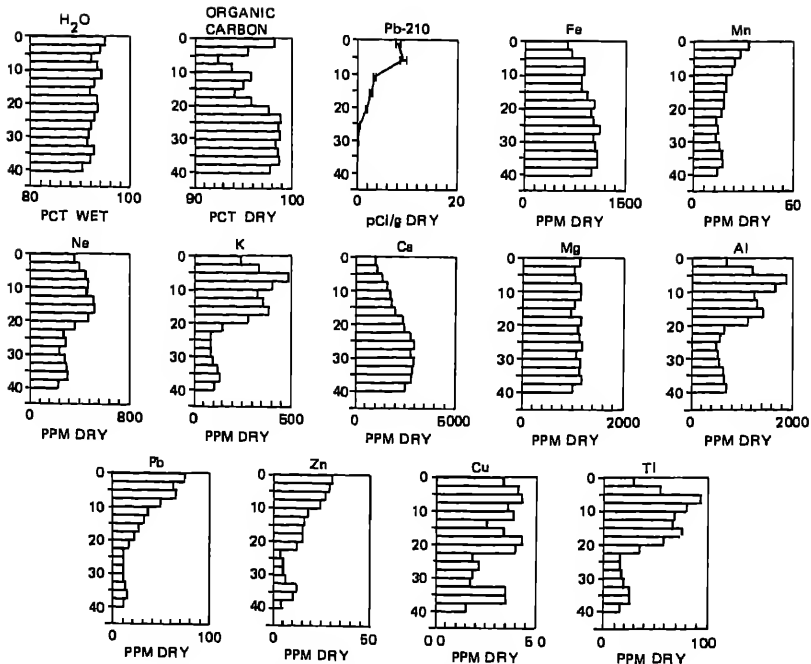
FIGURE 9.18 Chemistry of a hollow peat core from Big Heath, Mount Desert Island, Maine. Water table at about 5 cm. PPM DRY, parts per million, dry; pCi/g DRY, picocuries per gram, dry; PCT. DRY, percent dry; PCT. WET, percent wet. (From Norton 1983.)
