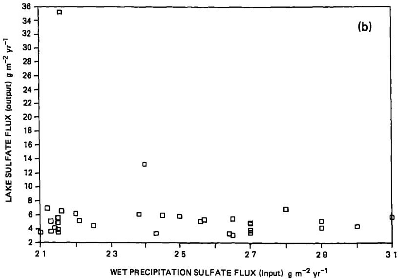
FIGURE 7.1 (a) Comparison of sulfate input fluxes to lakes from wet-only deposition with sulfate output fluxes from lakes in the northeastern United States and eastern Canada. (b) A similar plot for lakes in Massachusetts only.
