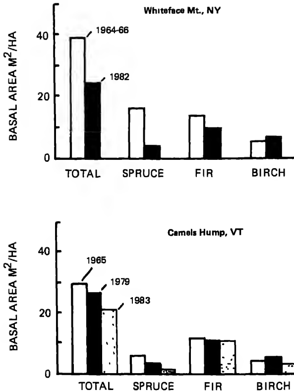
FIGURE 6.7 Basal area changes in major species at Whiteface Mountain, New York, and Camels Hump, Vermont. Basal area values include live trees of >10-cm dbh at Whiteface Mountain and of >2-cm dbh at Camels Hump. Data are for stands above 900 m at Whiteface and above 880 m at Camels Hump. (After Siccama et al. 1982 and Scott et al. 1984). 1983 Camels Hump data are from Ph.D. thesis of H. Whitney, Department of Botany, University of Vermont (unpublished).
