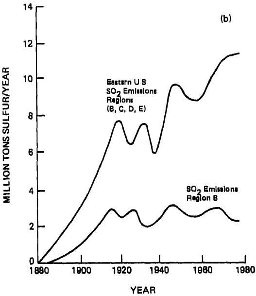
FIGURE 1.5 100-year trends in indices that may be related to acid deposition.
