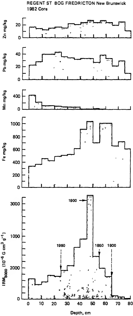
FIGURE 9.23 Magnetic and chemical stratigraphy from a hummock peat core (1982) from Regent Street Bog, Fredrickton, New Brunswick; dating by increments. IRM is isothermal remanent magnetism in units of Gauss, centimeters cubed per gram. (From F. Oldfield, University of Liverpool, U. K., and K. Tolonen,
