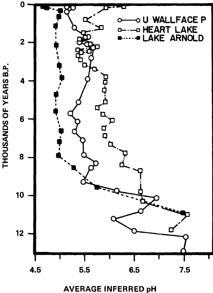
FIGURE 9.3 Weighted average diatom-inferred pHs for Heart Lake, Upper Wallface Pond, and Lake Arnold, Adirondack Mountains High Peaks Region. Averages were determined from index \alpha , index B, and multiple-regression equations. Each pH value was weighted by the standard error of each predictive equation. B. P. signifies before present. Whitehead et al. in press.
