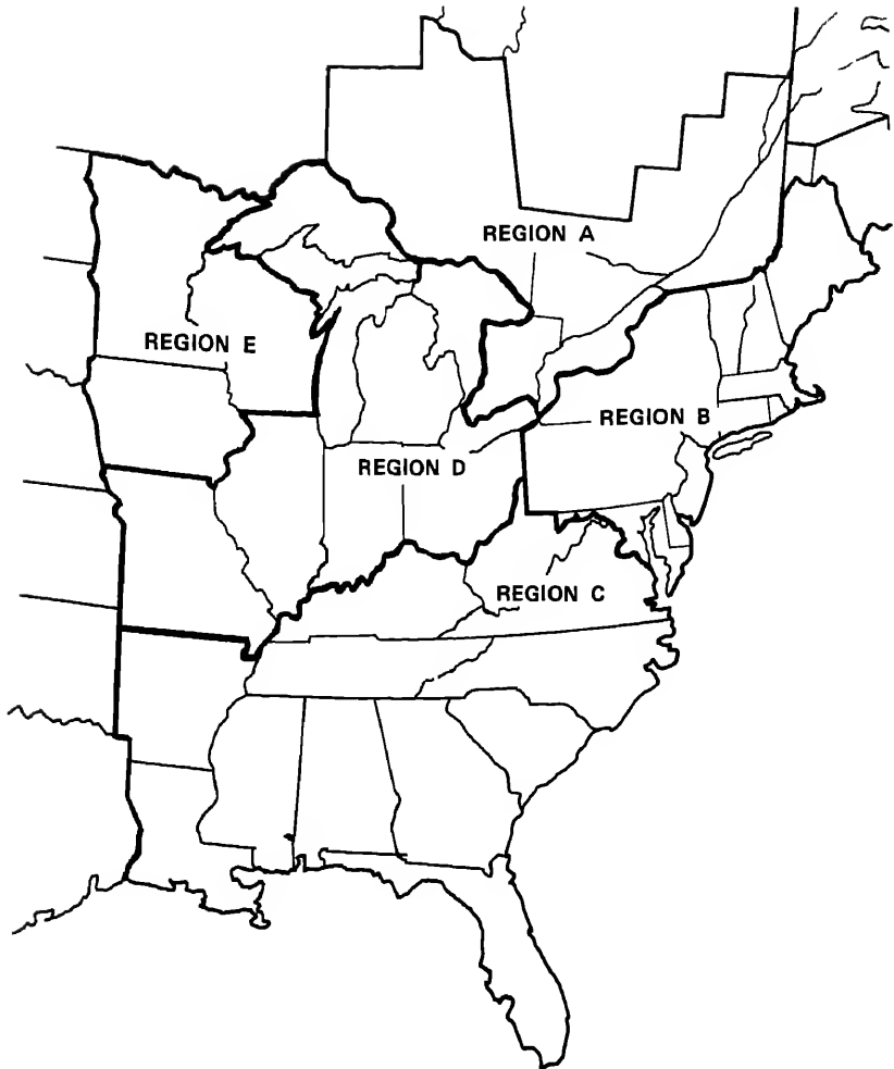
FIGURE 2.23 Regions in eastern North America selected for the study of regional trends in emissions.
