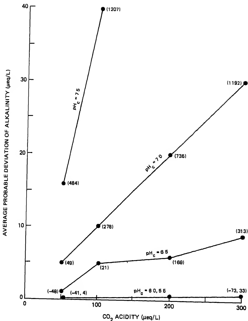
FIGURE 7.12 Average probable deviation to be expected for alkalinity calculated from free CO 2 acidity and colorimetric pH (pH c ). The deviation is obtained by varying pH c by ±0.2 unit and CO 2 acidity by ±5 µeq/L about assumed values. Numbers in parentheses next to the data points are actual calculated alkalinites.
