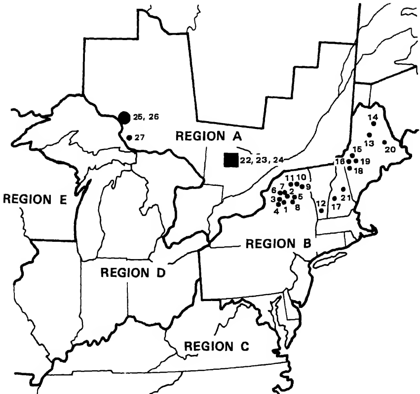
FIGURE E.1 Locations of 27 lakes in Regions A and B for which data on diatoms in sediments are available. The number next to each lake corresponds to the order in which it appears in Tables E.1 to E.5.
