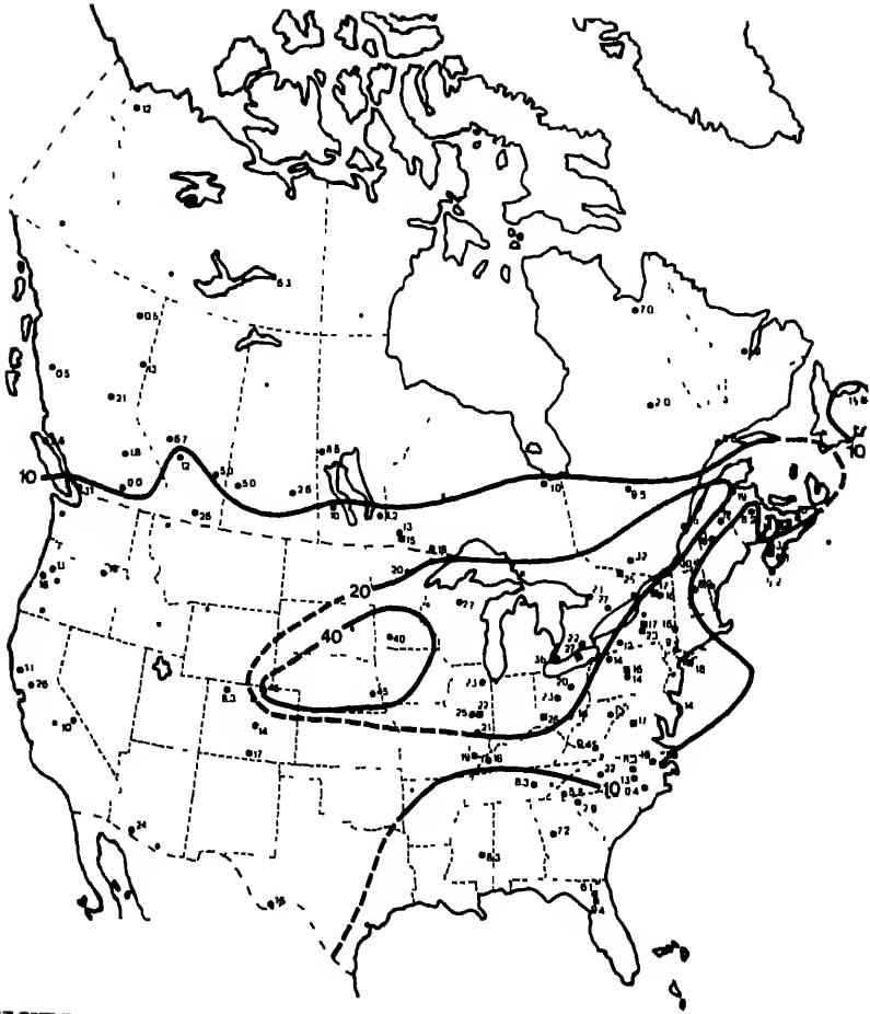
FIGURE 5.6 Spatial distribution of the precipitation-amount-weighted annual mean ammonium-ion concentration (micromoles per liter) in North America in 1980. Data from four networks are plotted: Canada, CANSAP (circles) and APN (squares); United States, NADP (circles) and MAP3S (squares). SOURCE: Barrie and Hales (1984).
