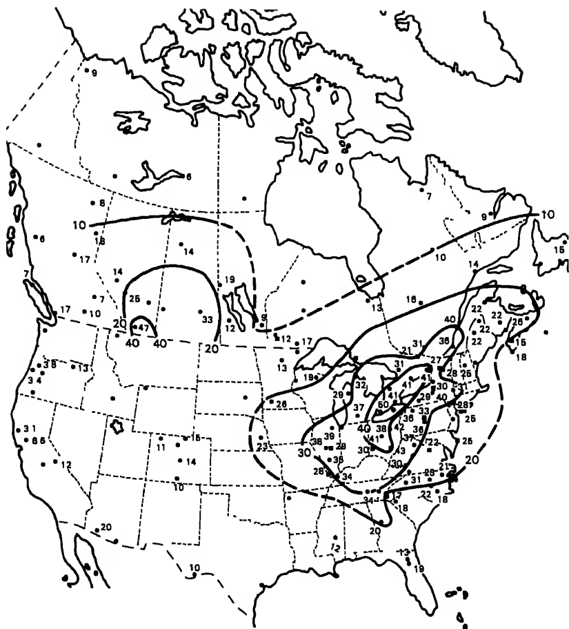
FIGURE 5.4 Spatial distribution of the precipitation-amount-weighted annual mean sulfate-ion concentration (micromoles per liter) in North America in 1980. Data from four networks are plotted: Canada, CANSAP (circles) and APN (squares); United States, NADP (circles) and MAP3S (squares). SOURCE: Barrie and Hales (1984).
