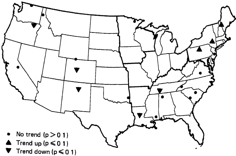
FIGURE 7.7 Trends in alkalinity at Bench-Mark stations having a mean alkalinity of less than 800 \mu\text{eq/L} . Regions B, C, D, and E are highlighted by darkened lines.
