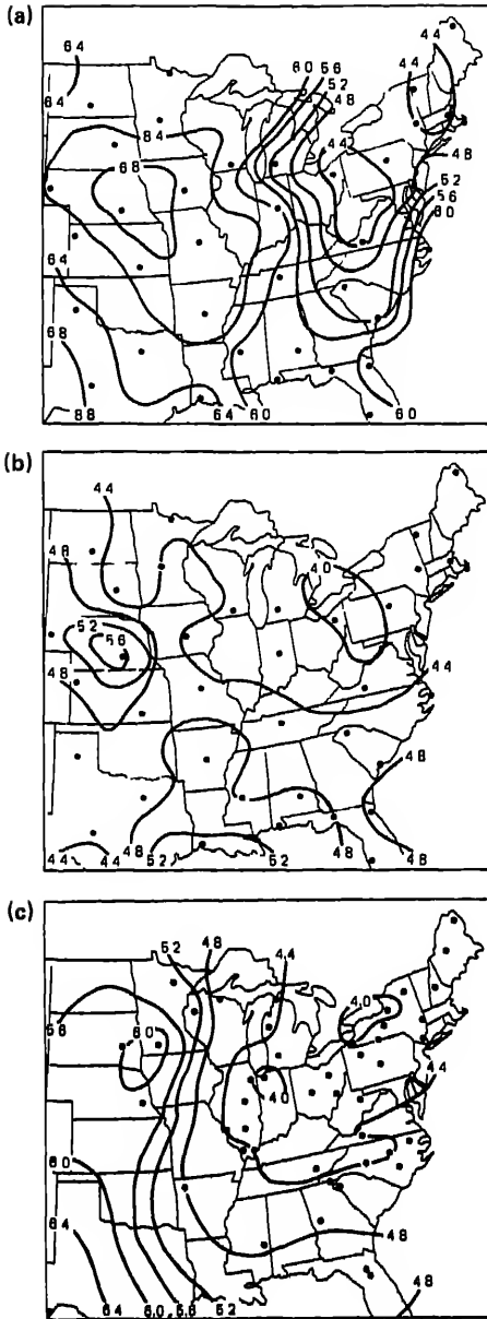
FIGURE 3.4 1955-56 pH distribution; (a) based on adjusted Junge data; (b) after correcting for assumed anomalously high concentrations of calcium and magnesium; and (c) September 1980 median pH distribution from National Acid Deposition Program network. See Chapter 5 for a detailed discussion of these data (Stensland and Semonin 1982).
