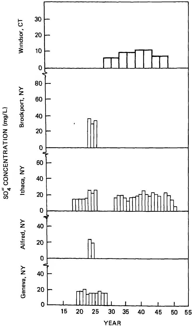
FIGURE 5.15 Sulfate concentration (milligrams per liter) in bulk precipitation samples for locations in the northeastern United States. The width of the bar designates the period of sampling. Adapted from Hidy et al. (1984). Data sources are listed in Table 1 of Hidy et al.
