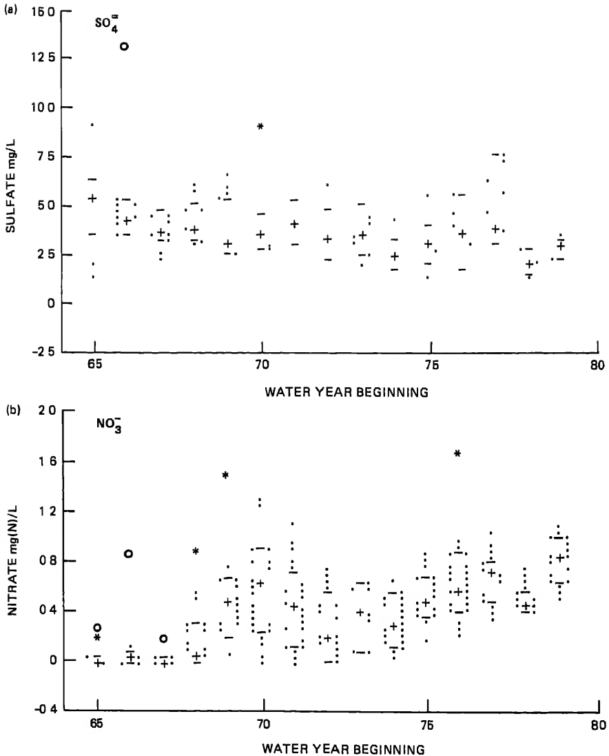
FIGURE 5.21 Box plots for precipitation chemistry at the Hinckley, New York, USGS site. (a) sulfate concentration, (b) nitrate concentration, (c) ammonium concentration, (c) pH. Data are from monthly bulk-deposition samples. The box encloses the middle 50 percent of the data for the year. The median value is denoted by a +. The dotted lines extending beyond the box give the range of all data for the year. The * and o symbols denote possible and probable outliers, respectively. SOURCE: Hidy et al. (1984).
