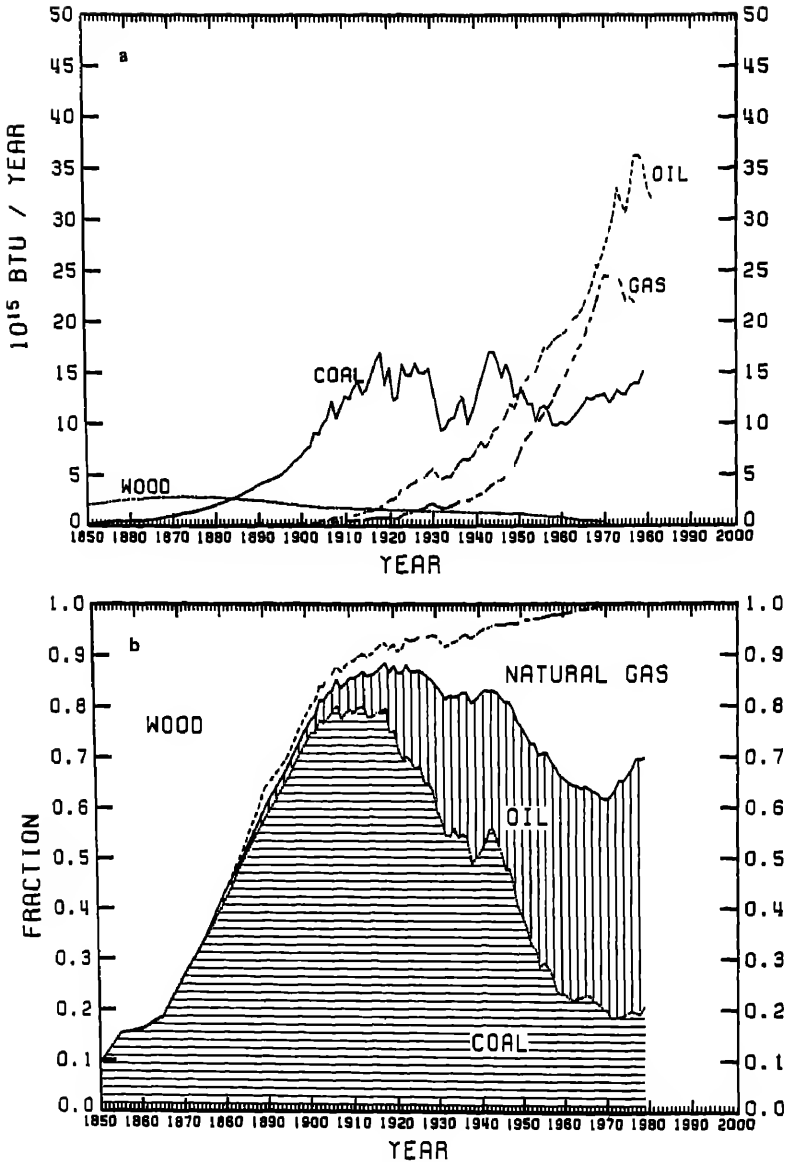
FIGURE 2.3 Trend for U.S. fossil fuel consumption since 1850. (a) Consumption by fuel type; (b) fraction of total energy by fuel type. Data for 1850 to 1880 from U.S. Bureau of the Census (1975); data from 1880 to 1932 from U.S. Geological Survey, Yearbooks (1880-1932); data from 1933 to 1980 from U.S. Bureau of Mines, Mineral Yearbooks (1933-1980).
