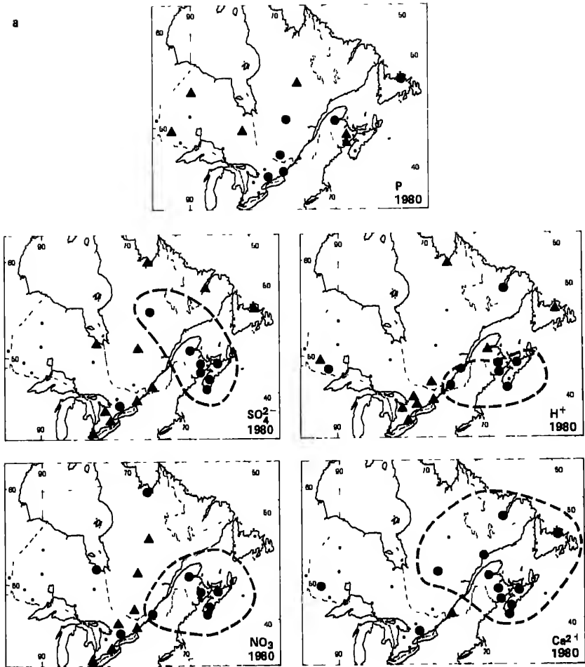
FIGURE 5.22 Comparison of the annual precipitation-weighted-mean concentrations of sulfate, hydrogen, nitrate, calcium, and precipitation amount (designated P in top panels in (a) to (e)) for (a) 1980; (b) 1981; (c) 1982 at eastern CANSAP stations. Filled circles denote maximum of three annual values; filled triangles denotes minimum.
