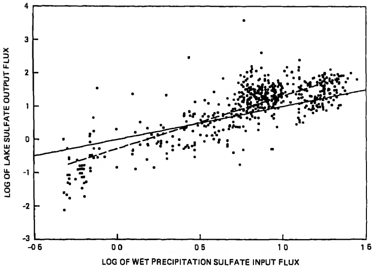
FIGURE 7.2 Comparison of the logarithm (base e) of sulfate fluxes to lakes from wet-only deposition with the logarithm (base e) of sulfate fluxes from lakes in the northeastern United States and eastern Canada. Solid line is the y = x line (i.e., condition in which sulfate flux from the lakes equals the sulfate flux to the lakes from wet-only deposition); dashed line is the line estimated from linear regression with slope of 1.593.
