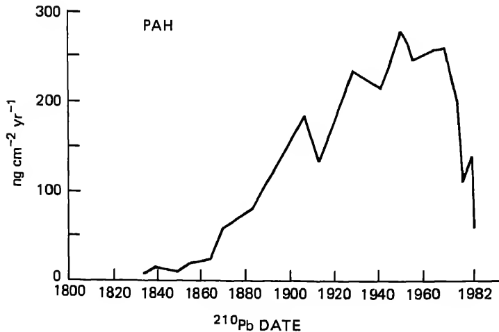
FIGURE 9.17 PAH and lead deposition rates for a core from Big Moose Lake, New York (lead data from Norton, unpublished; PAH data, courtesy of R. Hites, Indiana University, Bloomington, unpublished). Unit of mass given for PAH deposition is nanogram (ng) equal to one-billionth of a gram.
