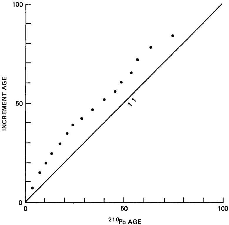
FIGURE 9.21 Increment age versus lead-210 age for a hummock peat core from Great Heath, Cherryfield, Maine (from Norton 1984).
