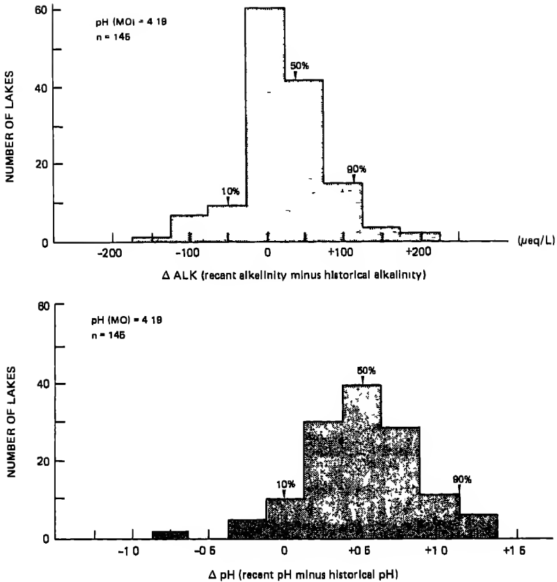
FIGURE 7.14 Changes in alkalinity and pH in Wisconsin lakes from the 1920s and 1930s to the 1980s, assuming a MO endpoint pH of 4.19.
