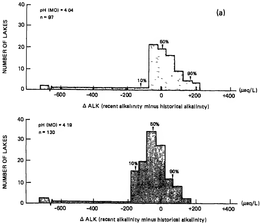
FIGURE 7.13 (a) Two scenarios for change in alkalinities of Adirondack lakes over five decades calculated from methyl orange endpoint pHs of 4.04 and 4.19. (b) Two scenarios for change in pHs of Adirondack lakes over five decades calculated from methyl orange endpoint pHs of 4.04 and 4.19.
