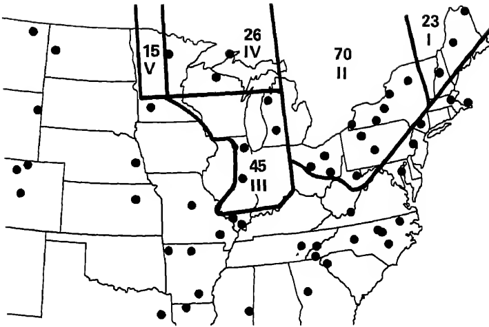
FIGURE 5.1 Map of five areas (indicated by roman numerals) used for comparing concentrations of various ions in wet-only deposition with those in bulk samples. The arabic numbers indicate the number of bulk sampling sites within each area. The NADP sites are indicated by circles. Bulk-measuring sites are distributed uniformly about the areas but are not co-located with NADP sites. See also Table 5.2.
