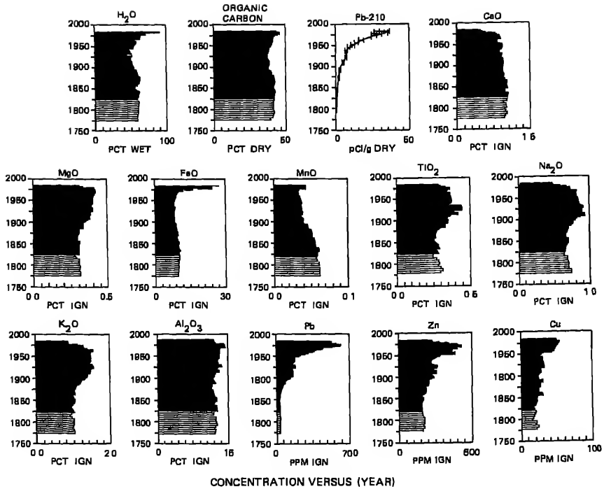
FIGURE 9.25 Concentrations versus year for various chemical species in Big Moose Lake (core 2). See caption, Figure 12, for definitions. Unpublished data from D. Charles (Indiana University) and S. Norton (University of Maine).
