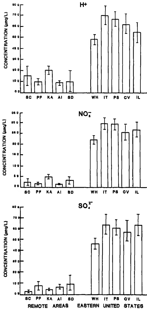
FIGURE 5.12 Comparison of the volume-weighted-mean concentration and the upper and lower error estimates among five sites in remote areas and five sites in the eastern United States. Remote sites: San Carlos, Venezuela (SC); Poker Flat, Alaska (PF); Katherine, Australia (KA); Amsterdam Island, Indian Ocean (AI); and Bermuda, Atlantic Ocean (BD). Eastern United States sites: Whiteface Mountain, New York (WH); Ithaca, New York (IT); State College, Pennsylvania (PS); Charlottesville, Virginia (CV); and Champaign, Illinois (IL). SOURCE: Galloway et al. (1984).
