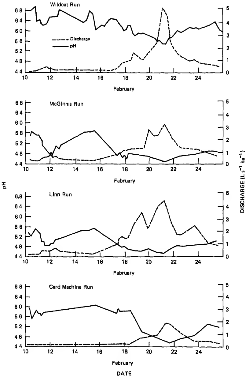
FIGURE 8.4 Changes in pH and discharge (in liters per second per hectare) over time for four streams on Laurel Hill, south central Pennsylvania. Source: Sharpe et al. (1984).
