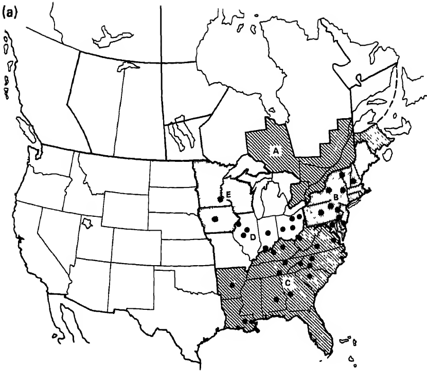
FIGURE 4.4 (a) Locations of 35 sites at rural airports for determination of visibility (1949-1983). (b) Locations of 15 rural sites of the NASN for determination of concentrations of airborne sulfate (1965-1978). Designated areas A-E represent the 5 regions defined in Chapter 1 of this report.
