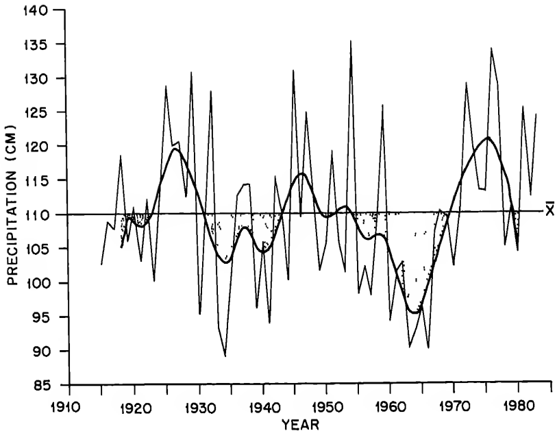
FIGURE 3.3 Annual precipitation in the Adirondack Mountains, New York. Horizontal line ( \bar{x} ) is the long-term average. Darker line shows low-frequency trends in the record (based on an 11-point binomial filter). Shaded areas indicate years of lower than average precipitation.
