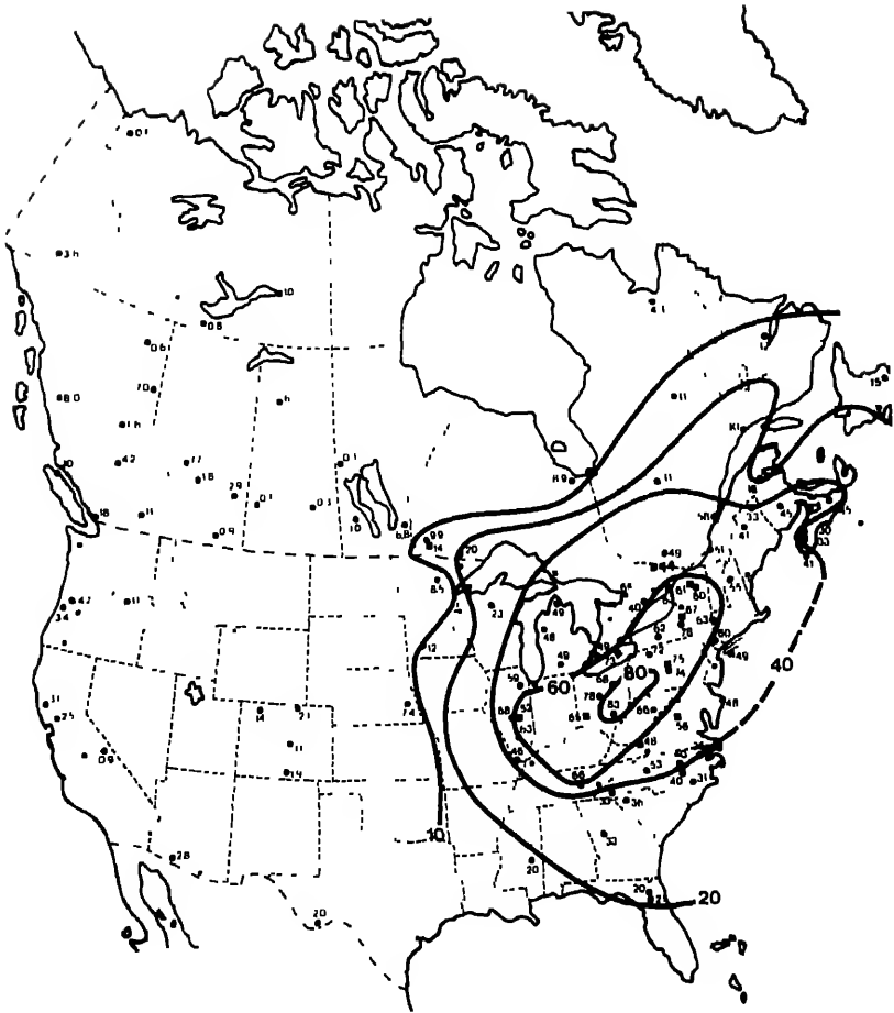
FIGURE 5.2 Spatial distribution of the precipitation-amount-weighted annual mean hydrogen-ion concentration (micromoles per liter) in North America in 1980. Data from four networks are plotted: Canada, CANSAP (circles) and APN (squares); United States, NADP (circles) and MAP3S (squares). SOURCE: Barrie and Hales (1984).
