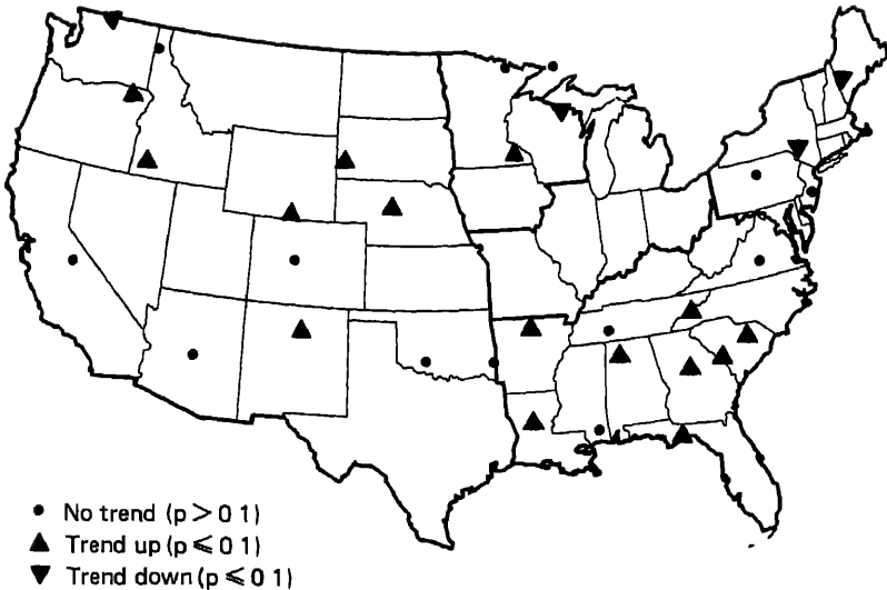
FIGURE 7.6 Trends in sulfate concentrations at Bench-Mark stations having a ratio of basin sulfate yield to basin sulfate deposition (wet-only) of less than 2.0. Regions B, C, D, and E are highlighted by darkened lines.
