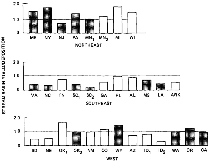
FIGURE 7.5 Ratio of stream basin sulfate yield to sulfate input from wet-only deposition at Bench-Mark stations that have ratios less than 2.0. Hatched bars correspond to streams with mean alkalinities less than 500 \mu\text{eq/L} . White bars correspond to streams with mean alkalinities greater than 500 \mu\text{eq/L} .
