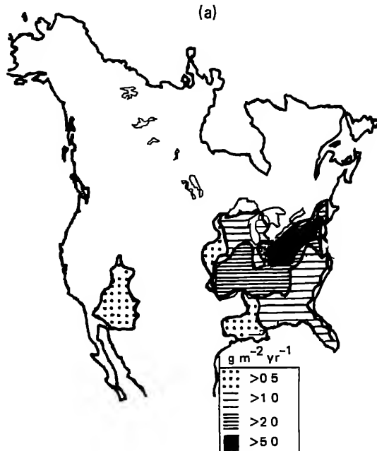
FIGURE 1.3 Comparison of spatial patterns between (a) \text{SO}_2 emission density ( \text{g m}^{-2} \text{yr}^{-1} ); (b) concentration of \text{H}^+ ( \mu\text{moles/L} ) in wet deposition; (c) concentration of \text{SO}_4^{2-} ( \mu\text{moles/L} ) in wet deposition; (d) concentration of sulfate aerosol ( \mu\text{g/m}^3 ); and (e) visible range (in miles).
