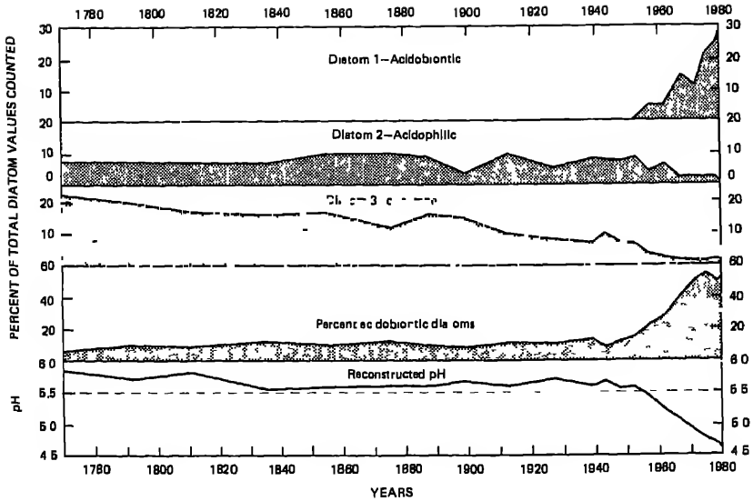
FIGURE 9.6 Reconstructed pH, percent of acidobiontic diatoms, and percent abundance of three diatom taxa, Big Moose Lake sediment core 2. Reconstructed pH is a weighted average of index \alpha , index B, and the multiple-regression equations shown in Figure 9.2. Weighting was based on the standard error of the three predictive equations (Figure 9.5). Diatom 1, Stauroneis gracillima , diatom 2, Anomoeoneis seriens var. bracysira , and diatom 3, Cyclotella stelligera , represent the dominant taxa in the core and occurred in subsets of 38 study lakes with mean pH values of 4.8, 5.9, and 6.8, respectively (Charles 1984). Percentage of euplanktonic taxa within the core followed the pattern of C. stelligera abundance very closely. Years are based on lead-210 dating (Figure 9.5).
