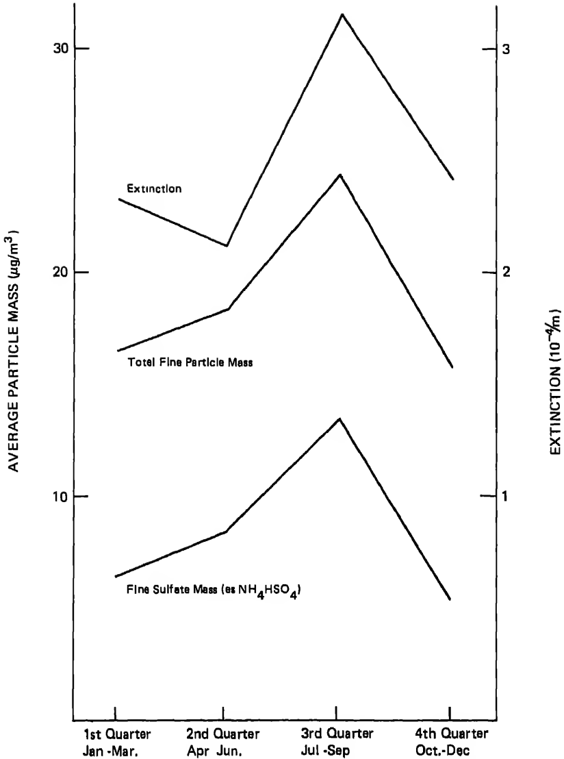
FIGURE 4.9 The seasonal patterns of fine-sulfate mass per unit volume, total fine-particle mass per unit volume, and light extinction for rural areas of the eastern United States. Fine-particle mass and fine-sulfate mass data are averages over five rural EPA dichotomous sampler sites (Will County, Illinois; Jersey County, Illinois; Monroe County, Illinois; Erie County, New York; and Durham County, North Carolina). The light-extinction data are averages over eight rural airports. SOURCES: Trijonis 1982, Trijonis and Yuan
