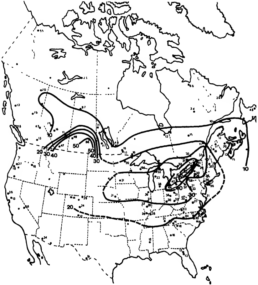
FIGURE 5.5 Spatial distribution of the precipitation-amount-weighted annual mean nitrate-ion concentration (micromoles per liter) in North America in 1980. Data from four networks are plotted: Canada, CANSAP (circles) and APN (squares); United States, NADP (circles) and MAP3S (squares). SOURCE: Barrie and Hales (1984).
