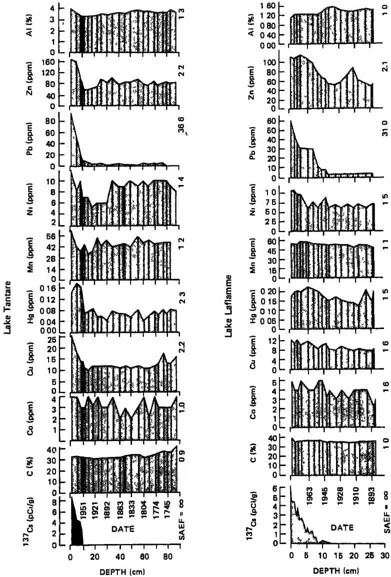
FIGURE 9.11 Sediment chemistry from lakes Tantare and Laflamme, Quebec, Canada (from Ouellet and Jones 1983). SAEF, sedimentary anthropogenic enrichment factor; pCi/g, picocuries per gram; ppm, parts per million. The value of SAEF is obtained by dividing the measured concentration by the background concentration. Thus, because the background value of picocuries per gram of cesium-137 is negligibly small, the SAEF value was assigned a value of
