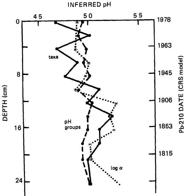
FIGURE 9.8 Comparison of downcore pH for Speck Pond, Maine, calculated from multiple-regression analysis of taxa and pH groups and from \log_{10} index \alpha (from Battarbee 1984). Lead-210 dates have been added to published figure; data from R. B. Davis, University of Maine, Orono, personal communication. CRS refers to Constant Rate of Supply model.
