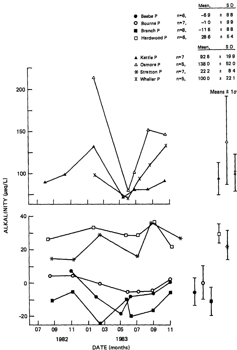
FIGURE 7.16 Monthly changes in alkalinity calculated from quality-assured data for lakes in Vermont.
