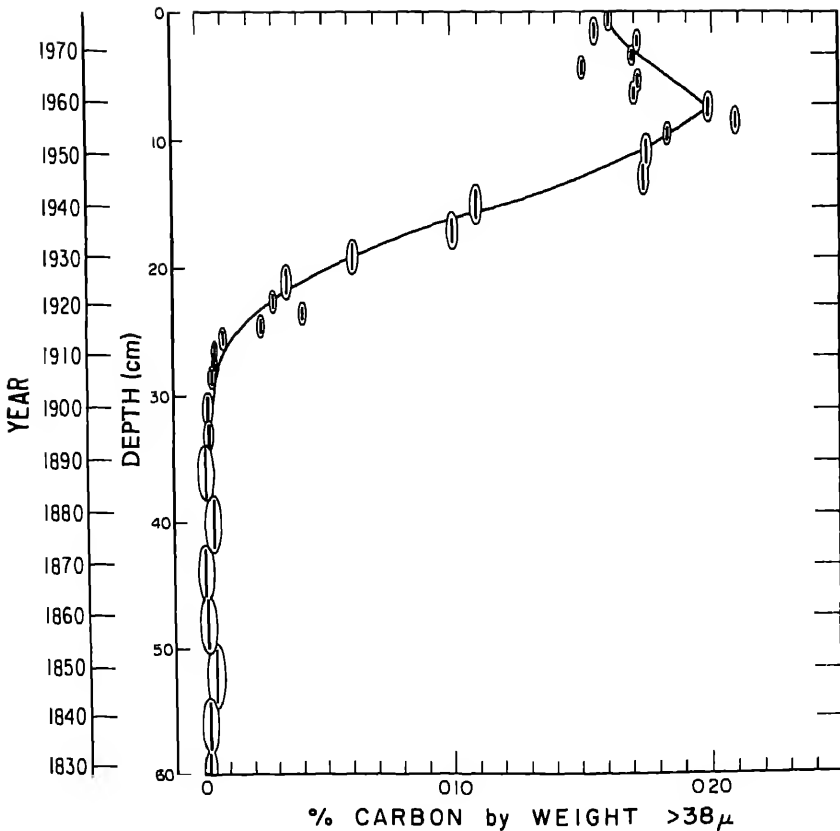
FIGURE 9.16 The record of concentration of charcoal particles in a sediment core from southern Lake Michigan. Particle sizes are greater than 38 microns (from Griffin and Goldberg 1981).
