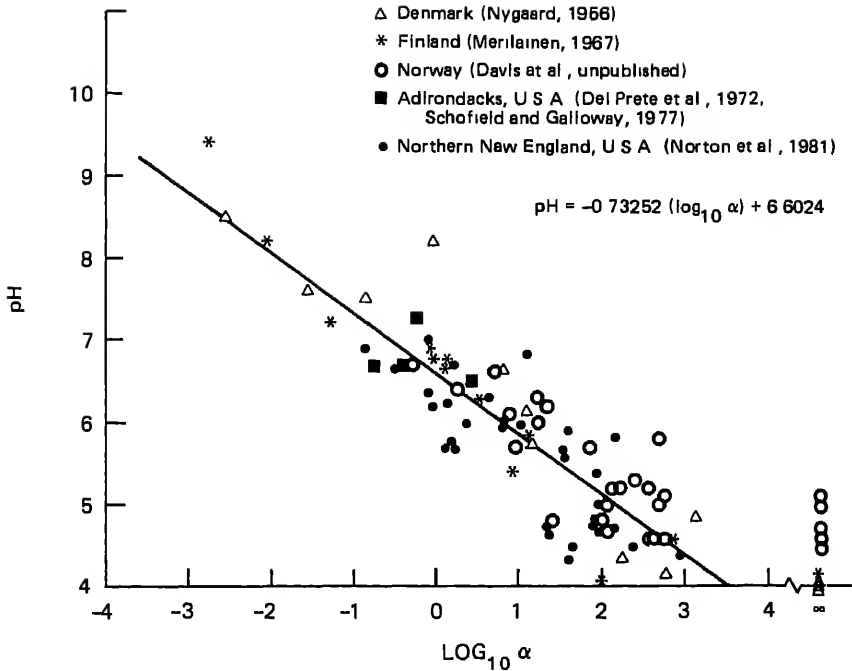
FIGURE 9.1 Logarithm of Nygaard's alpha index for surface sediment diatom assemblages versus lake surface water pH (Norton et al. 1981). Data for Norway are from R. B. Davis, F. Berge, and D. Anderson, University of Maine, Orono, unpublished data.
