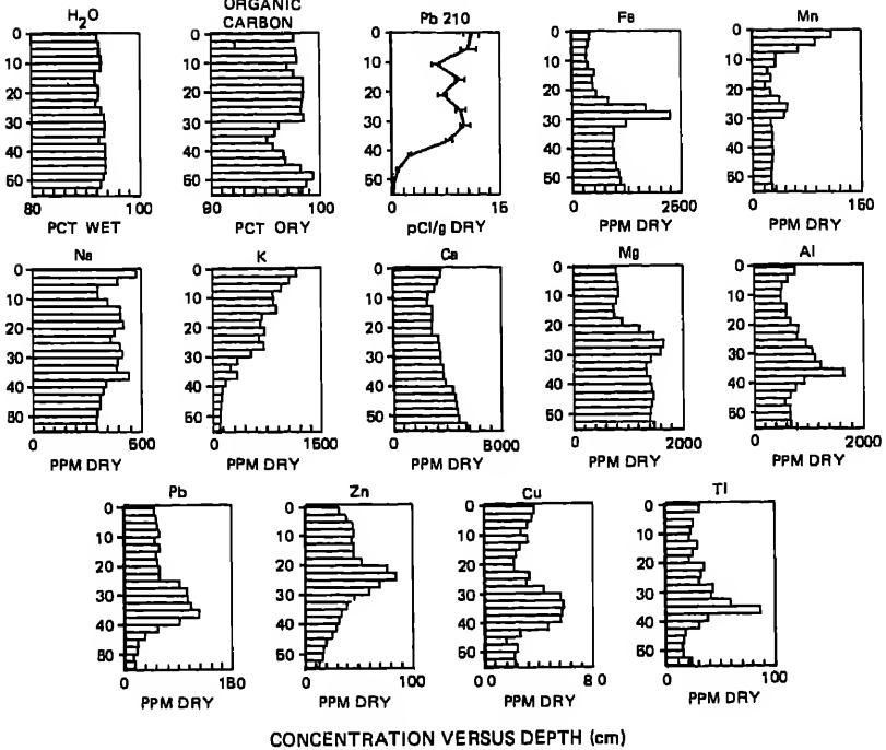
FIGURE 9.19 Chemistry of a hummock peat core from Big Heath, Mount Desert Island, Maine. Water table at about 30 cm. See caption, Figure 9.18 for definitions. (From S. A. Norton, University of Maine, Orono, unpublished data.)
