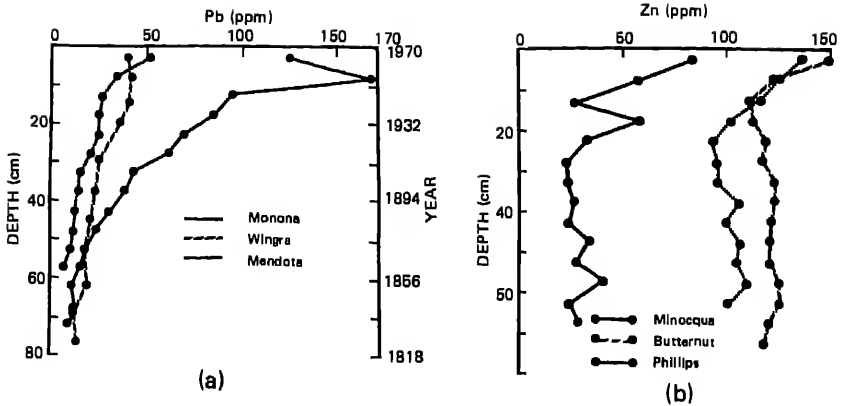
FIGURE 9.10 Vertical distributions of (a) lead and (b) zinc in selected Wisconsin lake sediments (from Iskandar and Keeney 1974).
