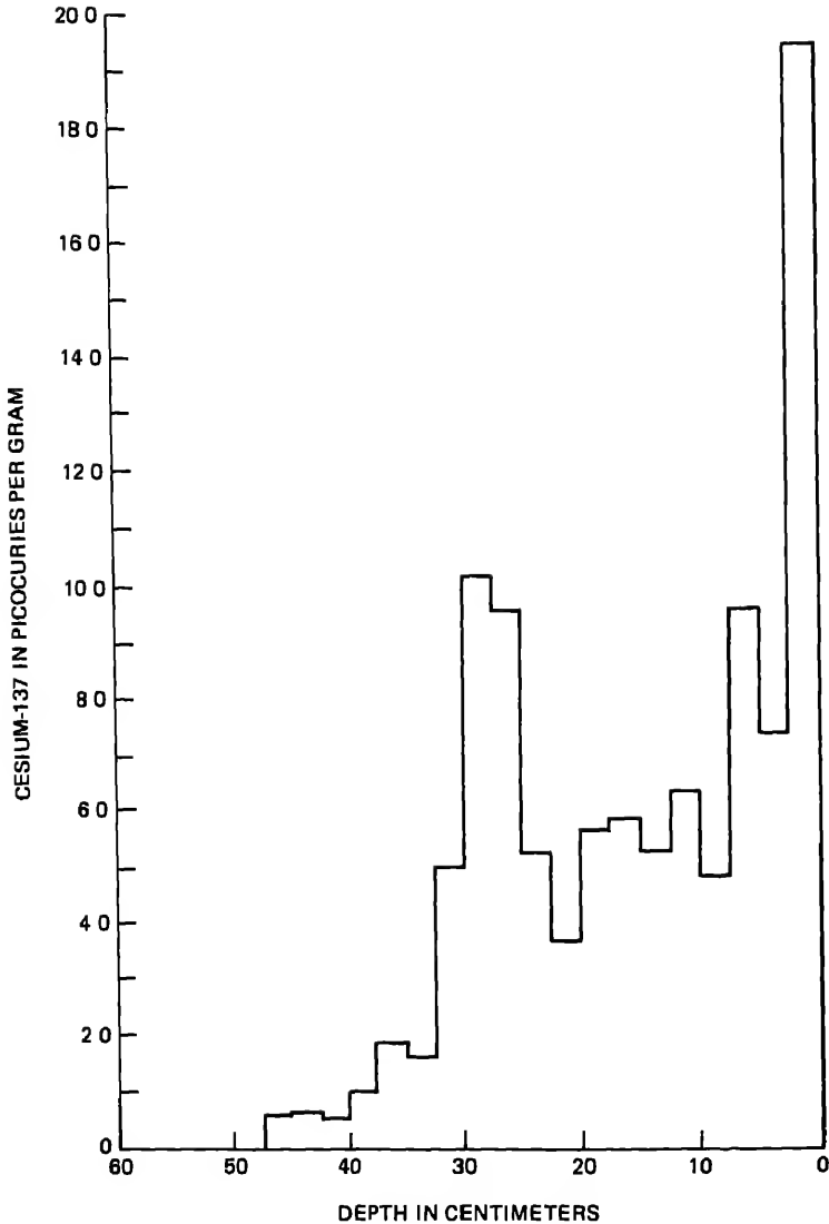
FIGURE 9.20 (a) Cesium-137 (Cs-137) activity in a hummock peat profile, Bull Hummock, in Bull Pasture Plain, New Brunswick (August 29, 1981) (from Olson 1983); (b) annual deposition of strontium-90 (Sr-90) in New York City. Cs-137 deposition = 1.7 \times Sr-90 deposition. (From Larsen 1984.)
