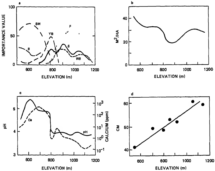
FIGURE 6.1 Altitudinal gradients in tree species and environmental characteristics at Camels Hump, Vermont. Curves are based on measurements at 11 elevations (except Figure 6.1(d) by Siccamo (1974) in 1964-1966. (a) Species importance value (based on basal area, density, and frequency) for sugar maple ( Acer saccharum Marsh) (SM); yellow birch ( Betula alleghaniensis Britt.) (YB); beech ( Fagus grandifolia Ehrh.) (B); red spruce ( Picea rubens Sarg.) (S); balsam fir ( Abies balsamea (L.) Mill) (F); white birch ( Betula papyrifera var cordifolia (Marsh) Regel) (WB). (b) Basal area of all live woody species of >2-cm dbh. (c) Soil pH (H 2 O) and exchangeable calcium (NH 4 OAC extraction) in the B horizon. (d) Growing season throughout fall collected by three to five rain gauges under the canopy at seven elevations. Amounts were measured weekly during the ice-free period during 1964-1966. (e) Maximum and minimum air temperature under the canopy. (f) Average number of frost-free days during 1964-1966.
