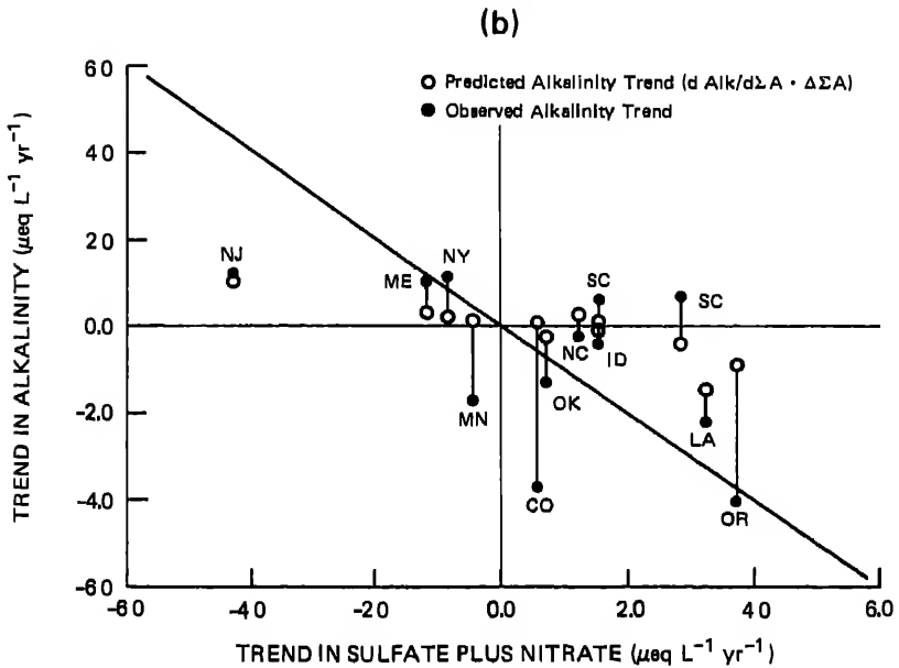
FIGURE 7.10 (a) Trend in alkalinity minus trend in base cations versus trends in sulfate plus nitrate. (b) Trend in alkalinity versus trend in sulfate plus nitrate.
