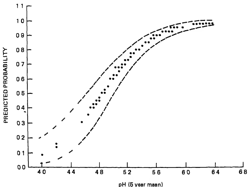
FIGURE 8.3 Predicted probability (and 95 percent confidence interval (dashed lines)) that status = 1 (fish community "healthy") as a function of mean 5-year pH. Status = 1 for lakes with fish community status rated 0 or 1. Source: Baker and Harvey (1985).
