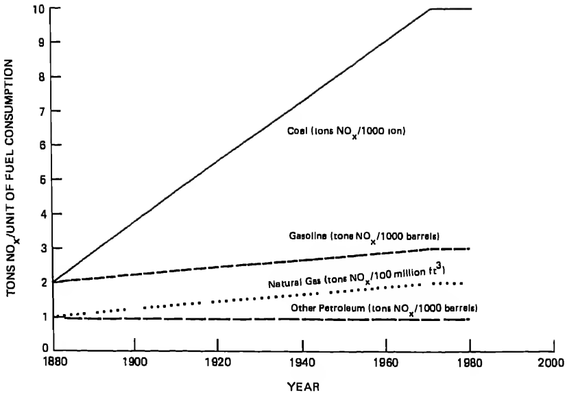
FIGURE 2.26 Trends in emission factors of nitrogen oxide by fuel type. Emission factors from the period of 1970 to 1980 were derived from data given from the U.S. Environmental Protection Agency (1977, 1978). For the period from 1880 to 1970, trends of historical emission factors were assumed to be linear, with slopes varying by fuel type.
