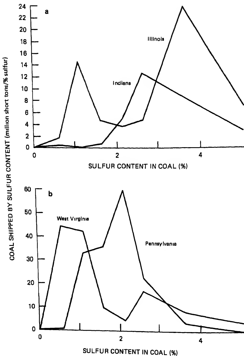
FIGURE 2.6 Distribution of coal sulfur content shipped from several coal-producing states. The data are averaged for the 9-year period from 1970 to 1978. SOURCE: Energy Information Administration 1981.
