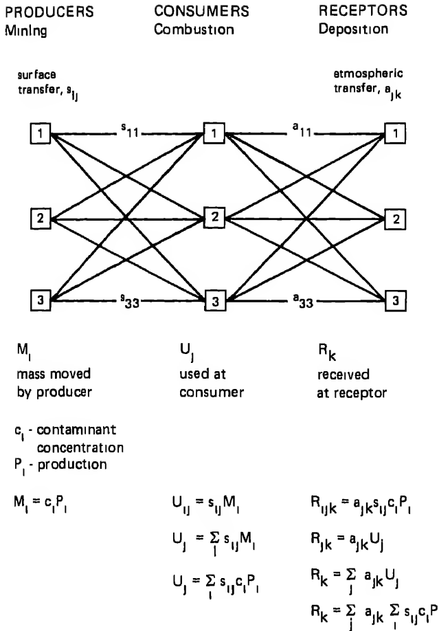
FIGURE 2.2 Schematic illustration of key matrices in the flow of material from the producer to the consumer to the receptor.
