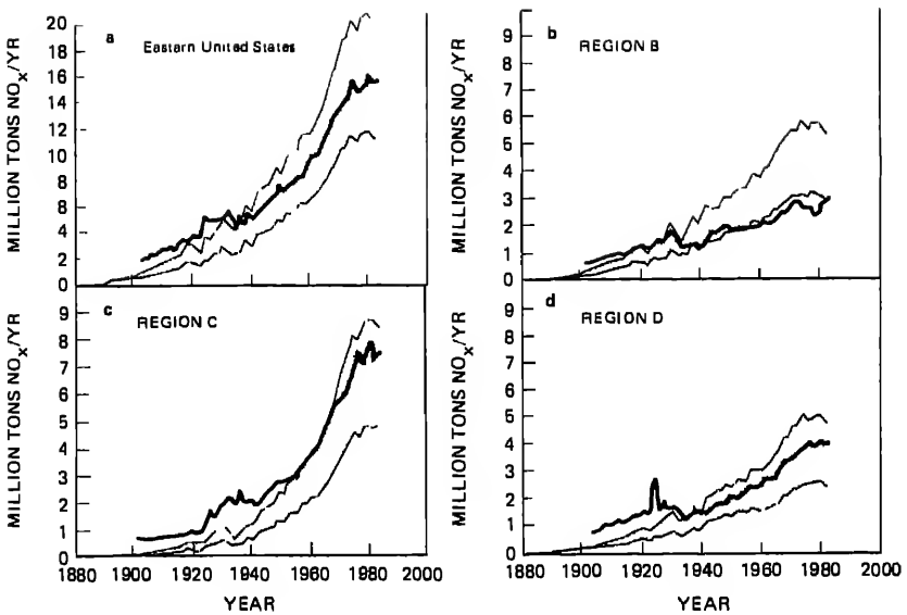
FIGURE 2.29 Comparison of estimates in nitrogen oxide emission trends reported in this chapter with the estimates of Gschwandtner et al. (1985) (dark lines) for (a) the eastern United States (Regions B, C, D, and E); (b) Region B; (c) Region C; (d) Region D.
