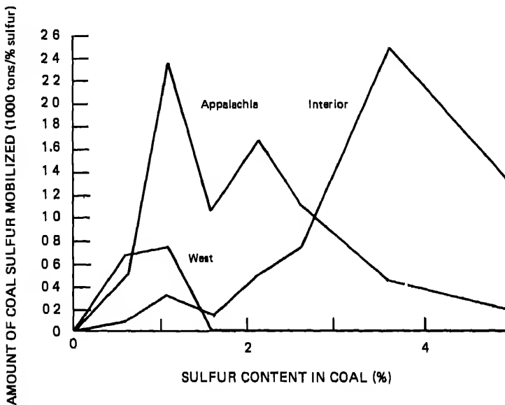
FIGURE 2.8 Coal sulfur distribution function for the three producing regions. The area under each curve is proportional to the amount of sulfur mobilized by each region. Data are averaged for the 9-year period 1970 to 1978. SOURCE: Energy Information Administration 1981.
