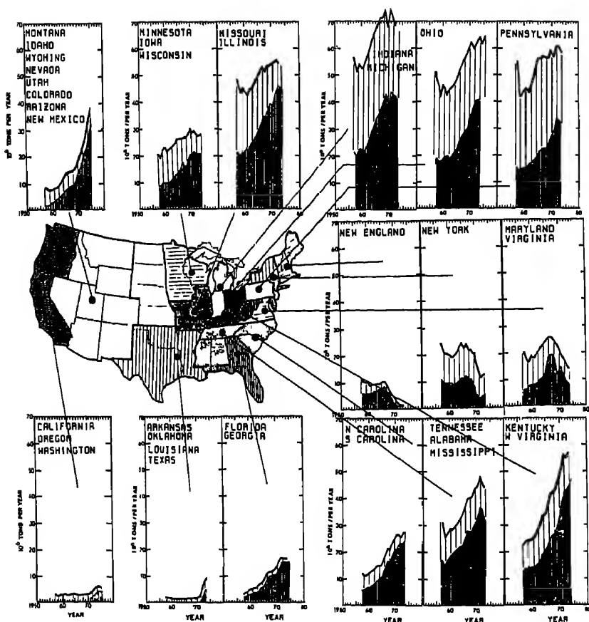
FIGURE 2.17 Trend of state-by-state consumption from 1957 to 1973. The shadings on the U.S. map represent groupings of states. The dark shading on the graphs represents electric utility consumption by state group. The light shading on the graphs represents all other coal-consuming sectors by state group. SOURCE: Husar et al. (1981).
